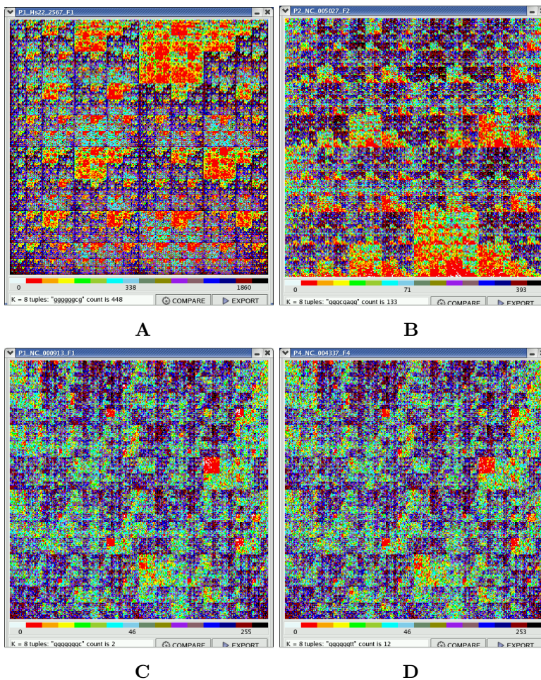
Fig. 1 2D portraits of the human chromosome 22 and the genomes of three bacteria. A. Human chromosome 22; B. Pirellula genome; C. Escherichia coli genome; D. Shigella flexneri 2a genome.
